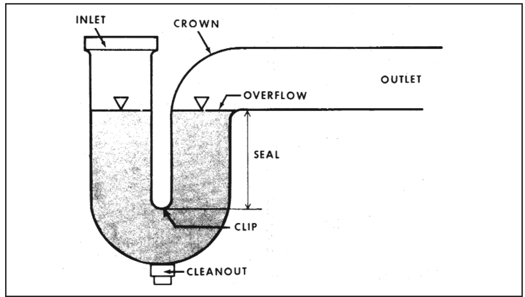
Figure 9.6. P-trap [1]
