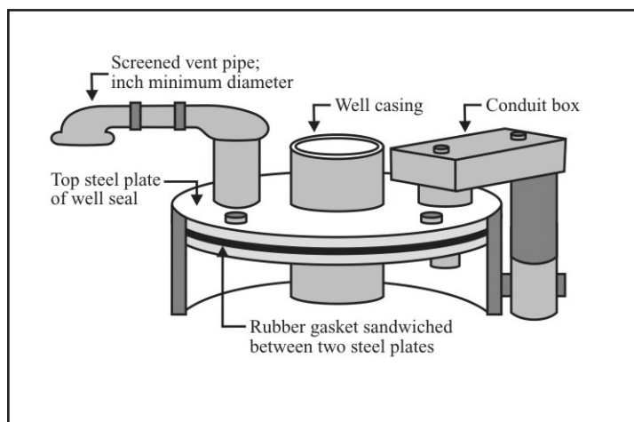
Figure 8.3. Well Seal
