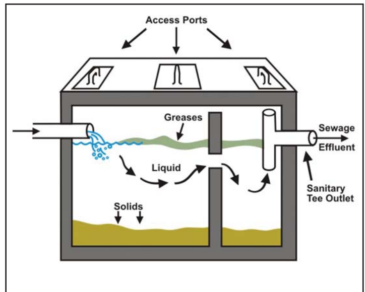
Figure 10.5. Septic Tank [9]
